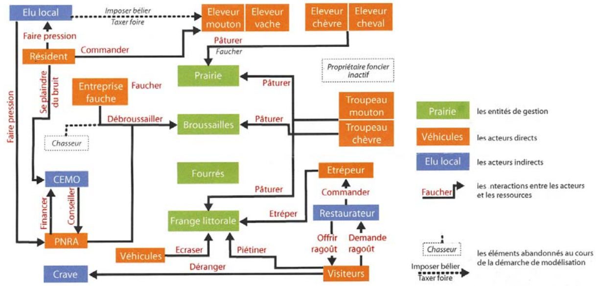
Flow-chart model of environmental behavior in Ouessant.
